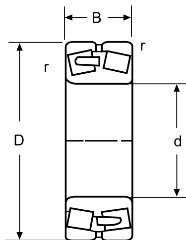
Cylindrical Bore 22300
