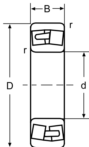
Cylindrical Bore 23000
