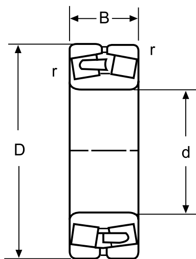
Cylindrical Bore 23100
