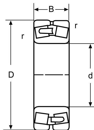
Tapered Bore 23100K
