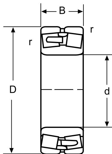
Cylindrical Bore 23200
