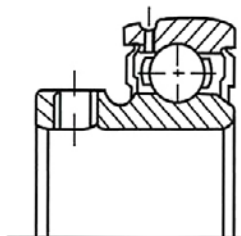
Seal type
